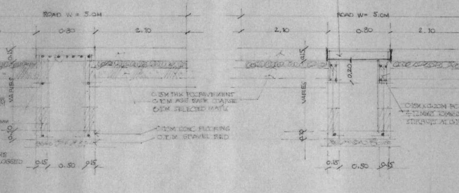
ROAD CROSS-SECTION AT FIXED COVER
