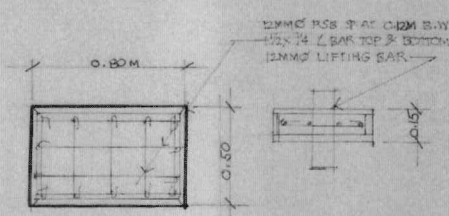
DETAIL OF M.H. COVER
