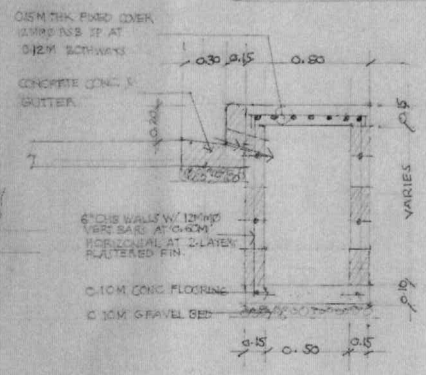
SECTION OF SIDEWALK
